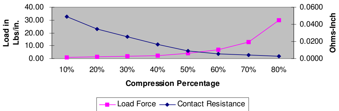
Contact Resistance and Compression-Load Deflection CF-78-20NR
