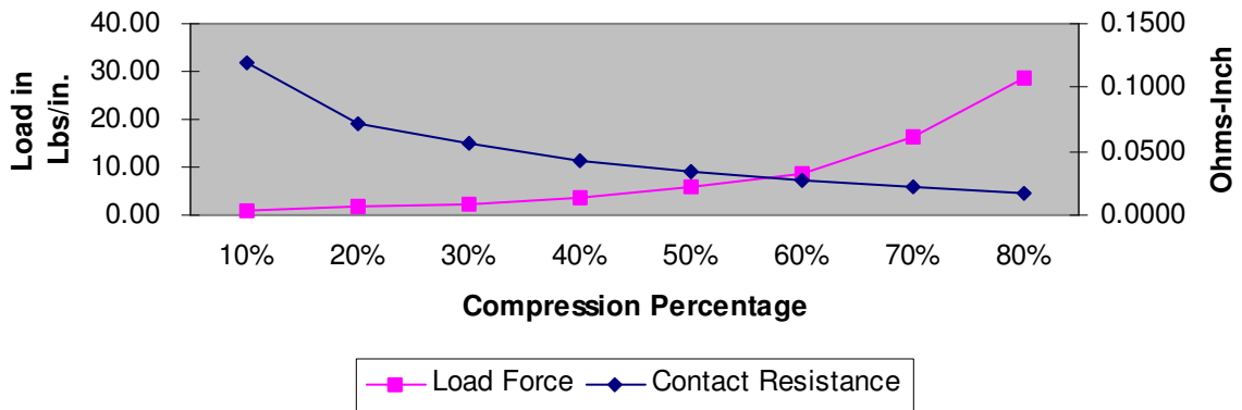
Contact Resistance and Compression-Load Deflection CF-78-14NR
