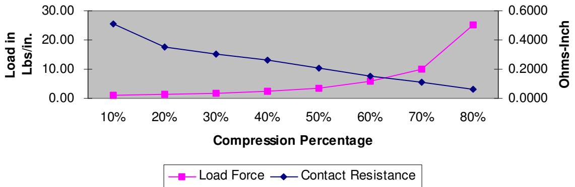
Contact Resistance and Compression-Load Deflection CF-78-20FR
